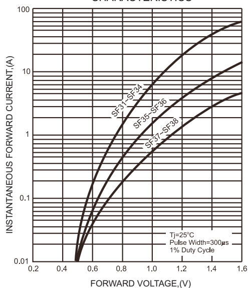
FIG.3-TYPICAL FORWARD CHARACTERISTICS
