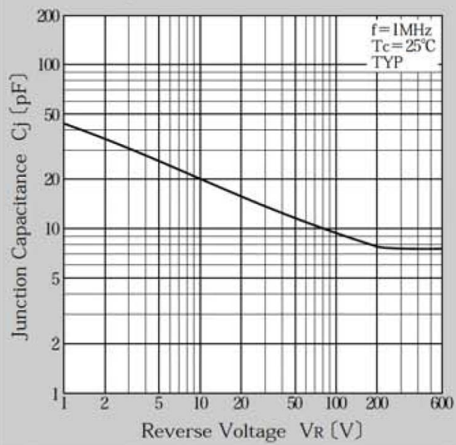
Junction Capacitance
