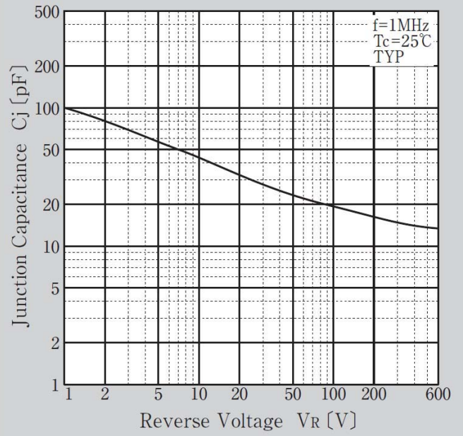
Junction Capacitance
