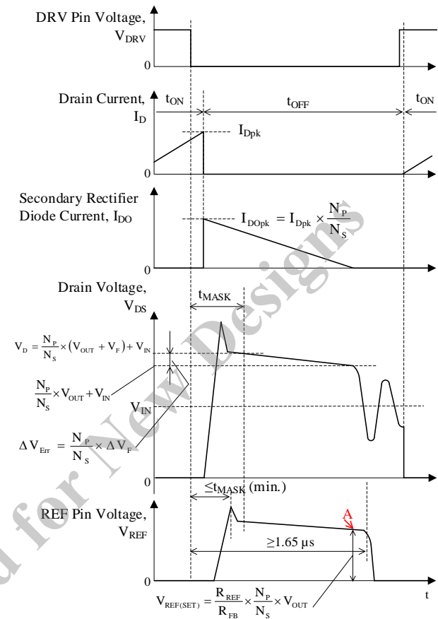
Figure 10-6. Detection Timing of Primary-side Winding Voltage
