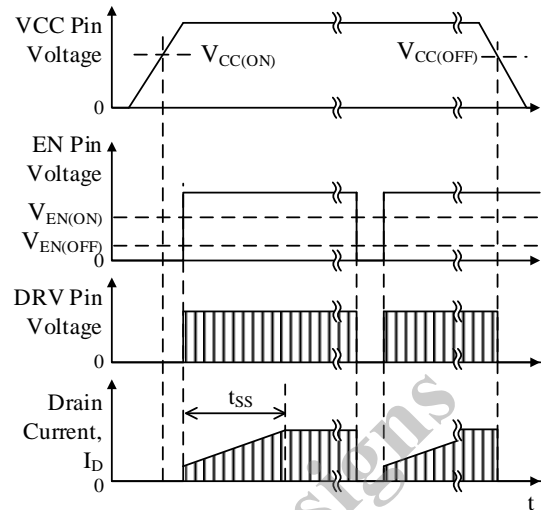
Figure 10-2. Operational Waveforms at Startup
