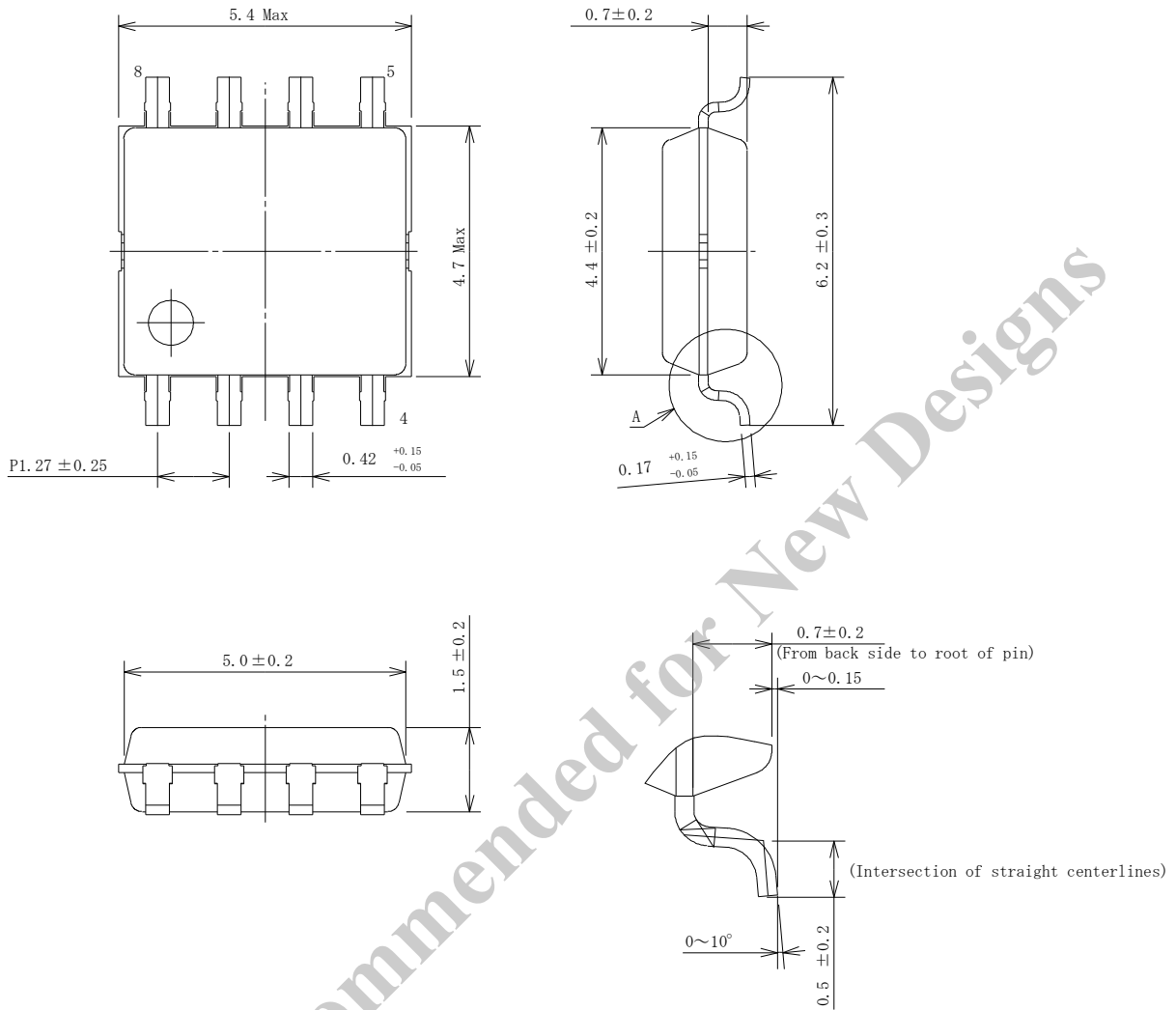
Enlarged view of A (S=20/1)
