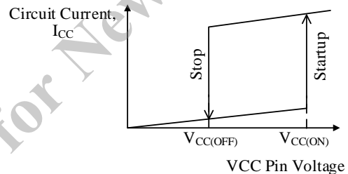
Figure 10-3. VCC Pin Voltage and Circuit Current ( V_{EN} \ge V_{EN(ON)} )
