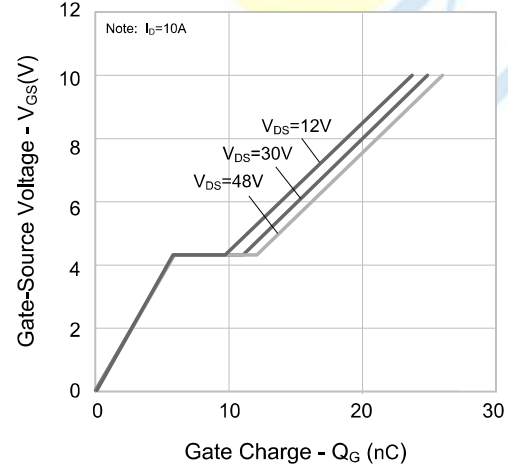
Figure 6. Gate Charge
