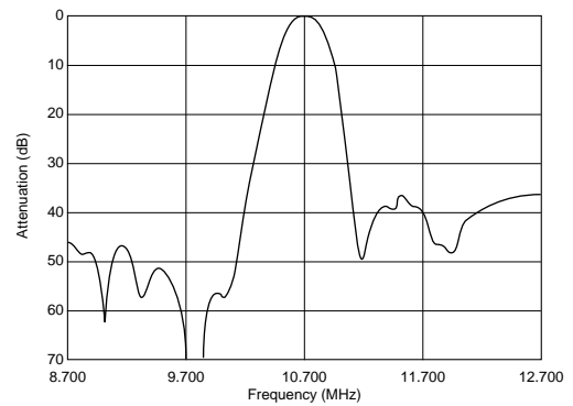
SFELA10M7FALL-B0
