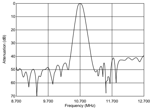
SFELA10M7JAXE-B0
