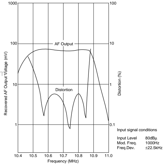
Frequency Characteristics
