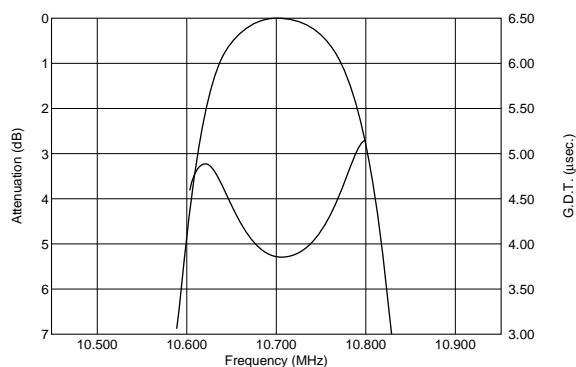
SFELA10M7HAA0-B0
