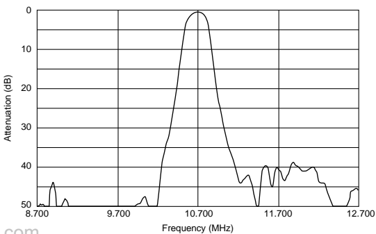
SF ECS10M7FA00-R0
