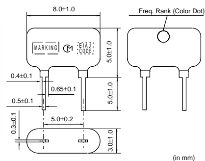
CDALA10M7C_Series
