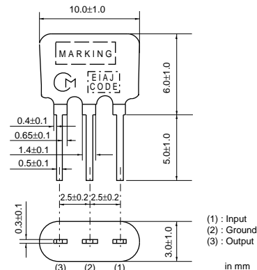
SFTLA10M7HA00-B0
