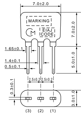
SFVLA10M7LF00-B0
