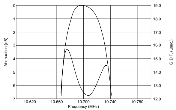
SFVLA10M7MF00-B0
