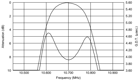
SF ECS10M7HA00-R0
