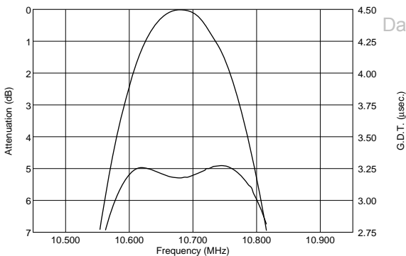
SFELA10M7HAXD-B0
