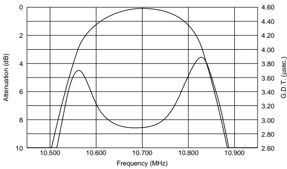
SF ECS10M7FA00-R0
