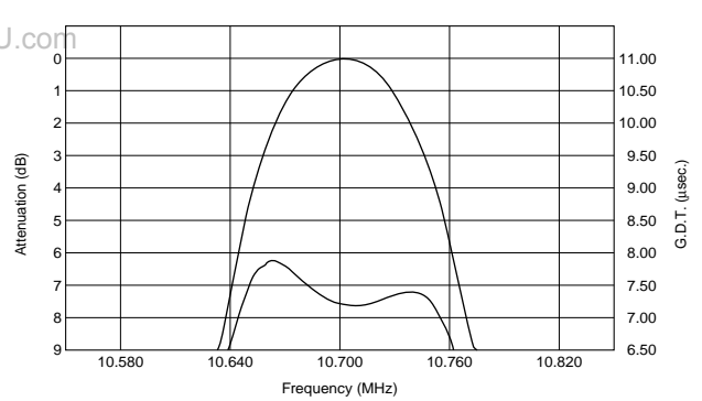
SFELA10M7LFTA01-B0
