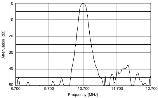
SF ECS10M7HA00-R0
