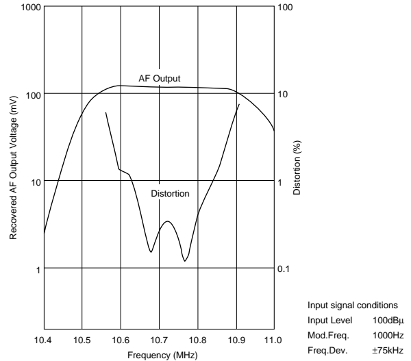
Frequency Characteristics
