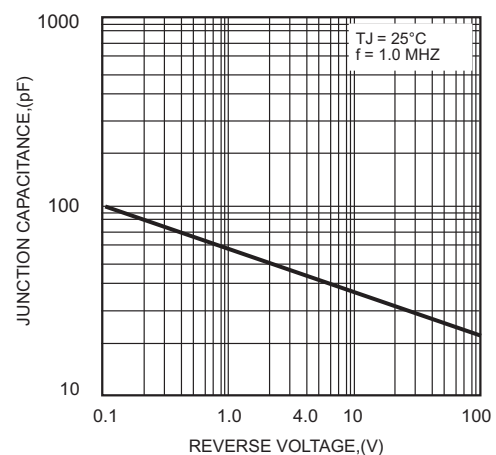
FIG.5-TYPICAL JUNCTION CAPACITANCE
