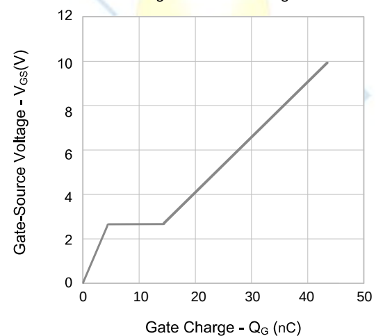
Figure 6. Gate Charge
