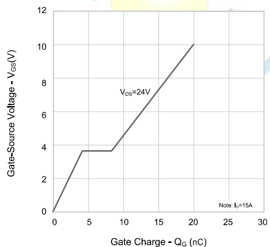
Figure 6. Gate Charge
