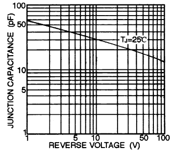
FIG. 4-TYPICAL JUNCTION CAPACITANCE
