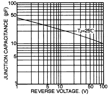
FIG.4-TYPICAL JUNCTION CAPACITANCE
