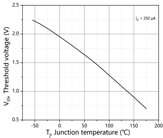
Figure 7. Threshold voltage
