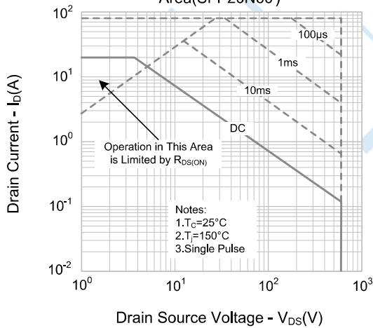
Figure 9-1. Max. Safe Operating Area(SFF20N60)
