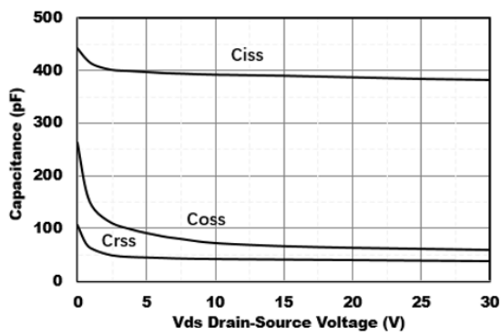
Figure 5. Capacitance Characteristics
