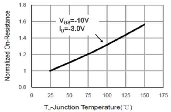
Figure 4. Drain-to-Source On Resistance
