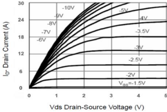
Figure 1. Output Characteristics
