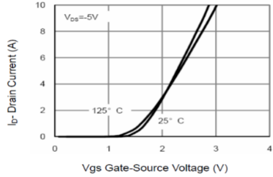
Figure 2. Transfer Characteristics
