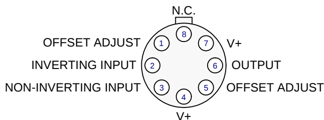
T PACKAGE
