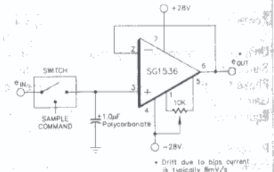
FIGURE 8 - LOW-DRIFT SAMPLE AND HOLD
