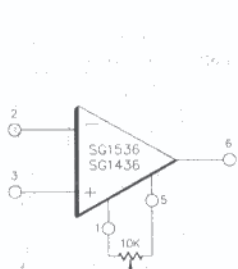
FIGURE 6 - VOLTAGE OFFSET NULL CIRCUIT
