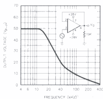
FIGURE 1 POWER BANDWIDTH
