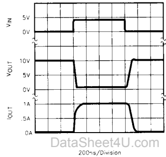
FIGURE 5. DYNAMIC RESPONSE WAVEFORM
