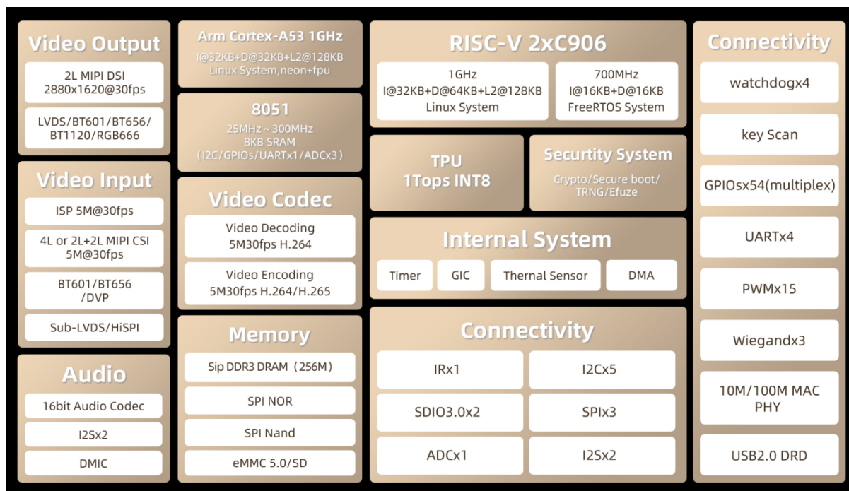
Figure 1- 1 SG2002 architecture diagram
