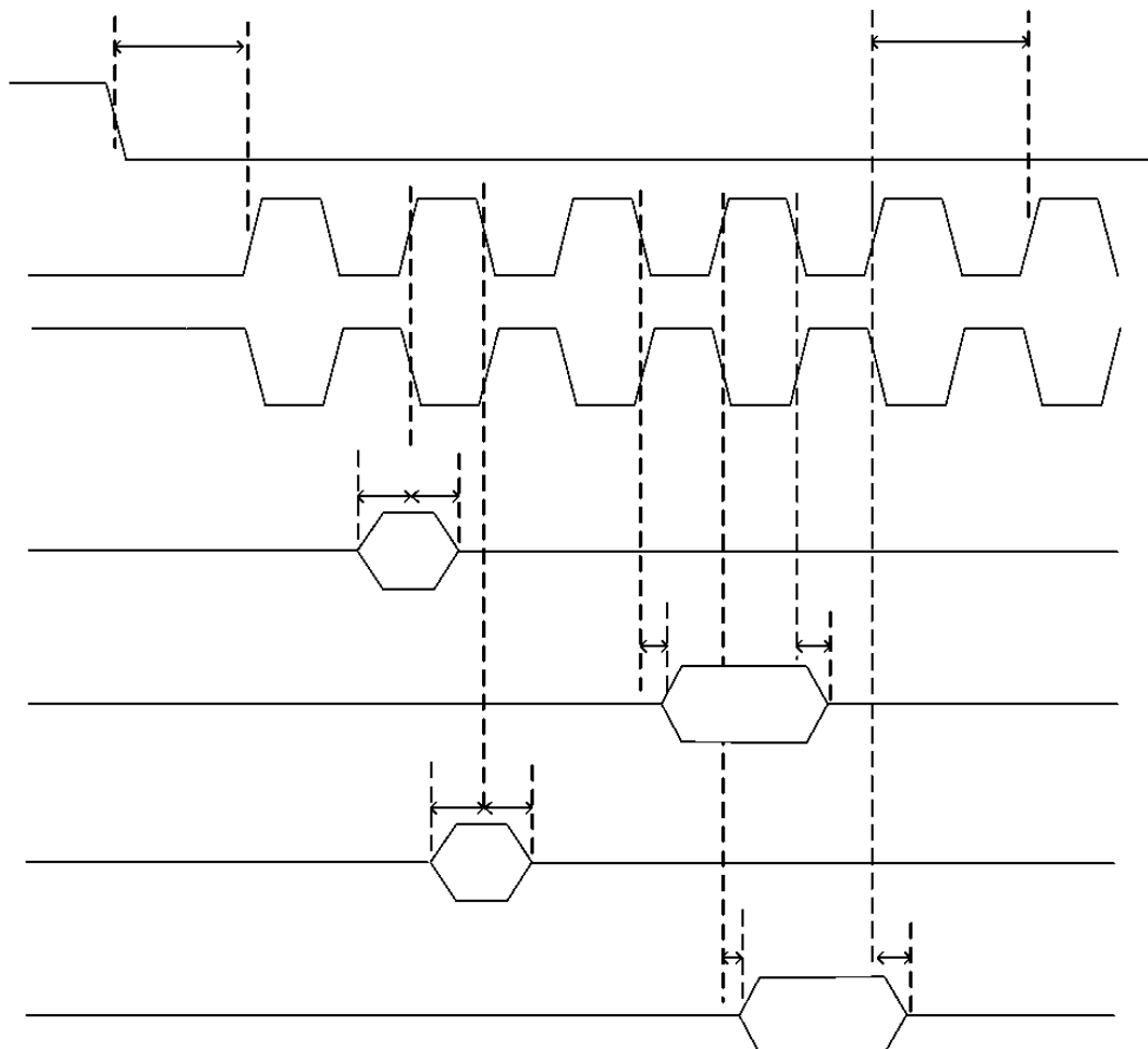
Figure 2-19 SPI Timing Diagram
