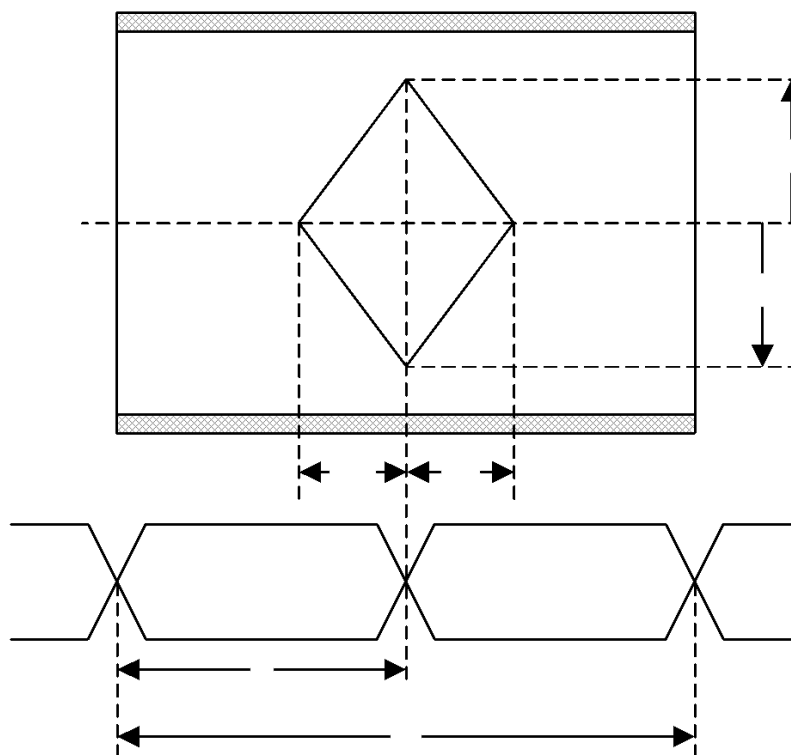
Figure 2-22 HiSPi Clock Data Timing Diagram
