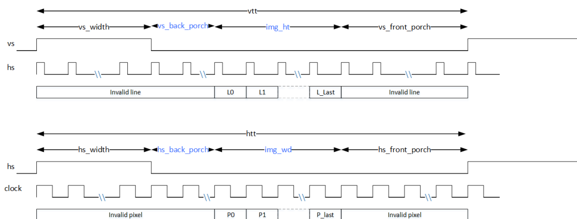
Figure 2-13 BT.601 Timing Diagram
