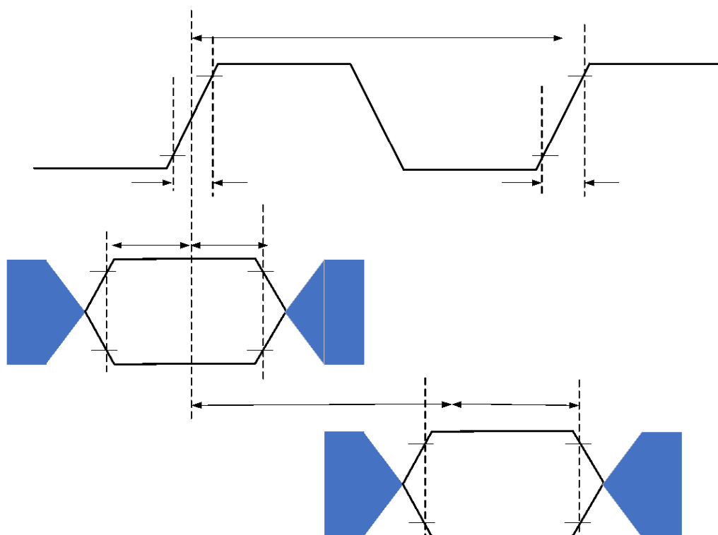
Figure 2-28 SDIO/MMC HS200 and SDR104 mode data command input/output timing diagram
