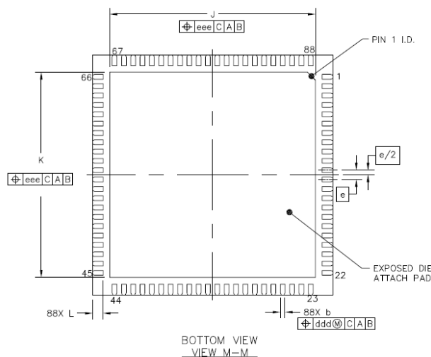
Figure 2-2 SG2002 Package external dimensions, bottom view
