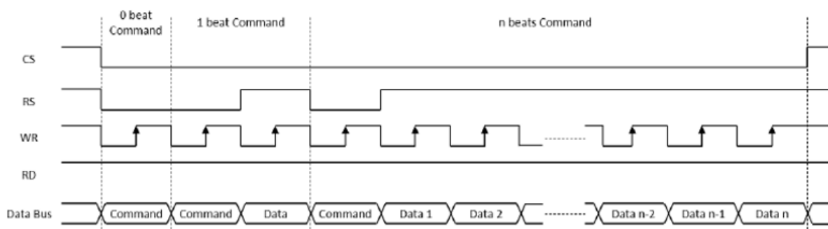
Figure 2-15 8080 Timing Diagram
