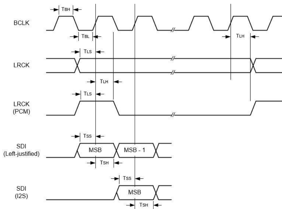
Figure 2-16 I2S & PCM Rx Timing Diagram
