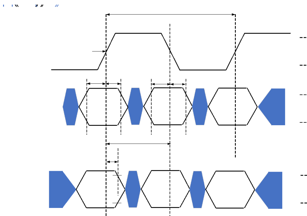
Figure 2-27 SDIO/MMC double edge DDR50 mode data input/output timing diagram
