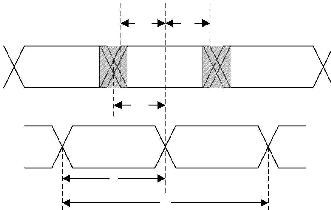
Figure 2-20 Timing Diagram of MIPI Rx Clock when 0.08\text{Gbps} \leq \text{Data Rate} \leq 1.5\text{Gbps}
