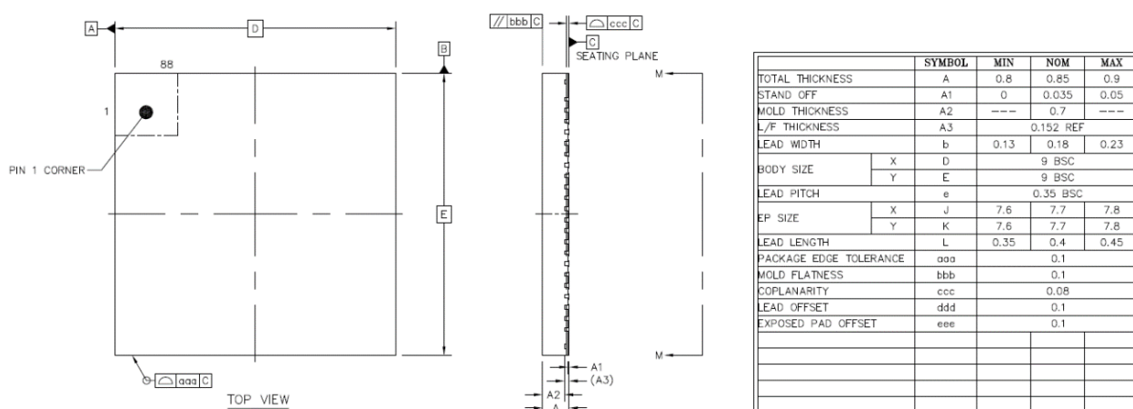
Figure 2-1 SG2002 package dimensions, top view
