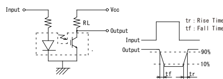
*1 Switching Time Measurement Circuit
