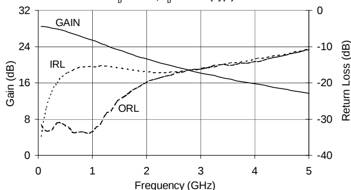
Gain & Return Loss vs. Frequency V_D = 3.25\text{ V} , I_D = 35\text{ mA} (Typ.)
