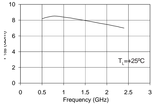
P_{1dB} vs. Frequency V_D = 2.7V , I_D = 20mA
