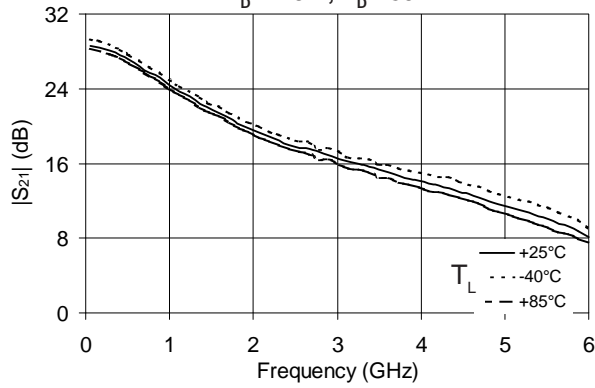
|S_{21}| vs. Frequency V_D = 4.9 \text{ V}, I_D = 80 \text{ mA}
