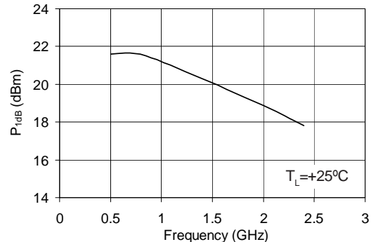
P_{1dB} vs. Frequency V_D = 4.9V , I_D = 80mA
