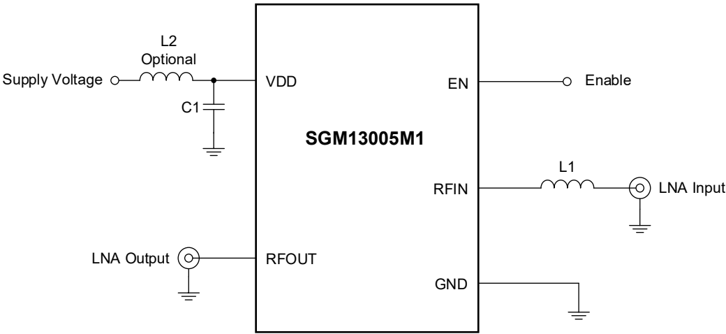
Figure 2. SGM13005M1 Typical Application Circuit
