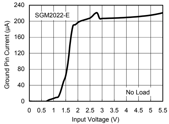
Ground Pin Current vs. Input Voltage
