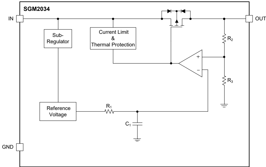
Figure 2. Block Diagram
