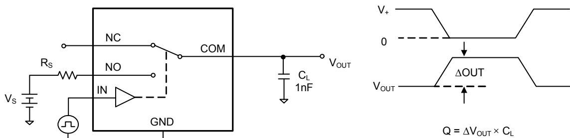
Test Circuit 7. Charge Injection (Q)
