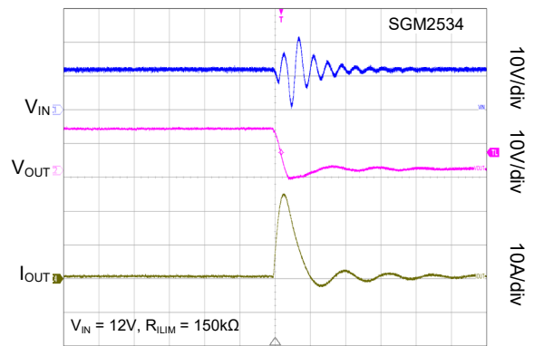
Time (2µs/div)
