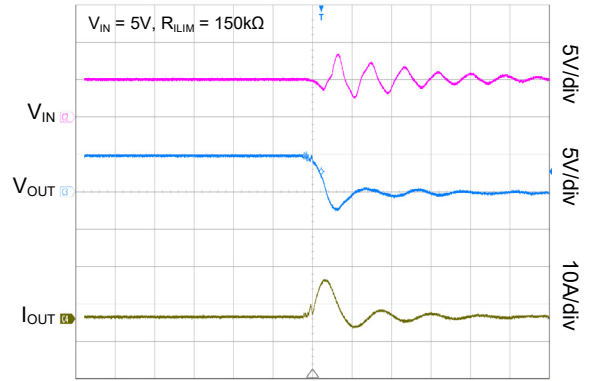
Time (2µs/div)
