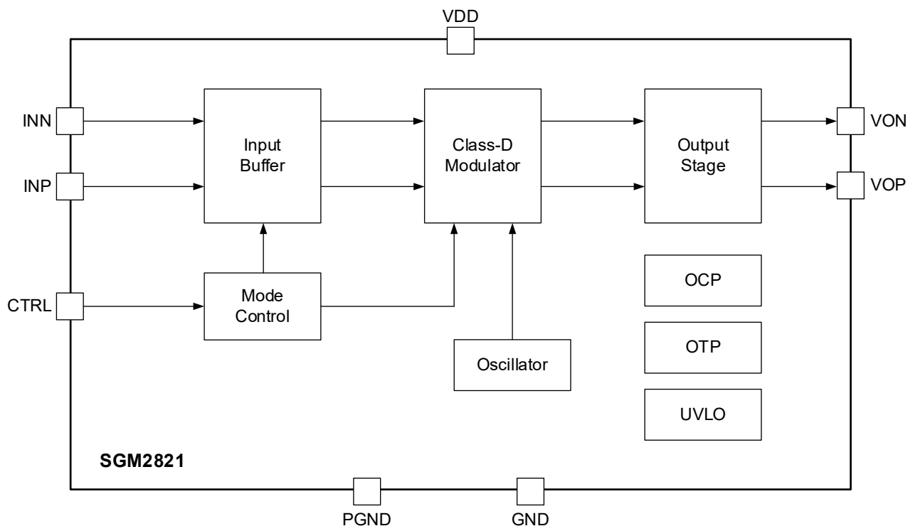
Figure 3. Block Diagram
