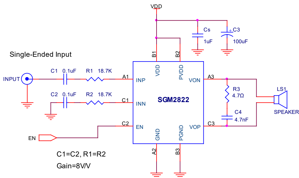
Figure 7. Single-Ended Audio Input Application
