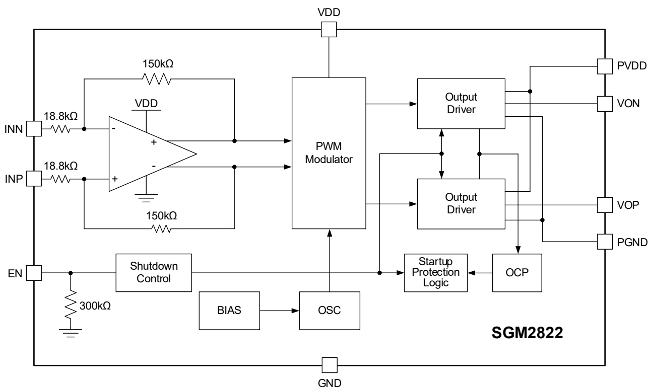
Figure 3. Simplified Function Block Diagram of SGM2822
