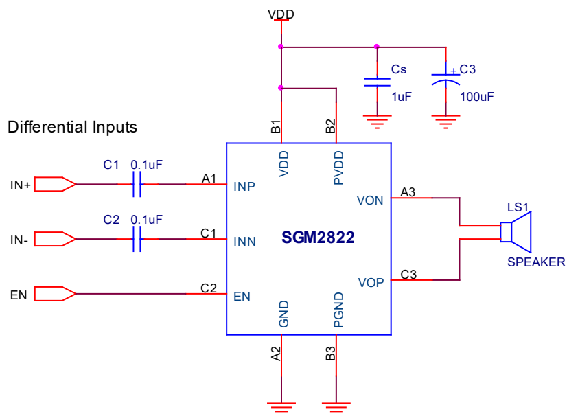
Figure 6. Differential Audio Input (for Mobile Phone Application)
