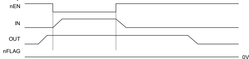
Figure 7. Slave Mode OTG
