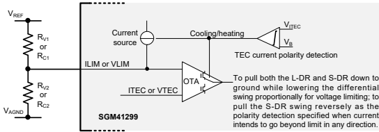
Figure 10. Voltage and Current Limit Circuit Architecture
