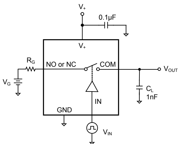
Test Circuit 3. Charge Injection
