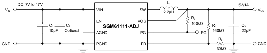
Figure 8. 5V Output Voltage Application of SGM61111-ADJ
