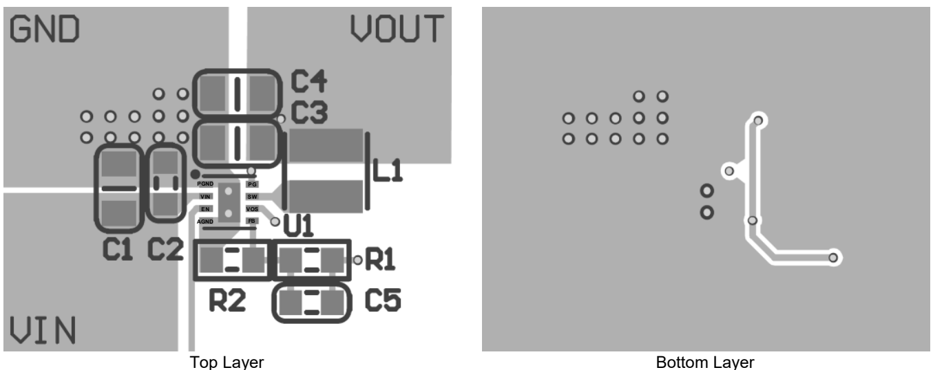
Figure 10. PCB Layout
