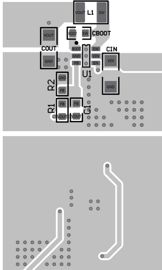
Figure 6. Suggested PCB
