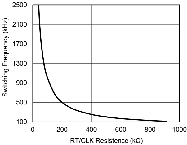
Switching Frequency vs. RT/CLK Resistance
