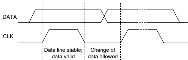
Figure 15. Bit Transfer on the Serial Interface
