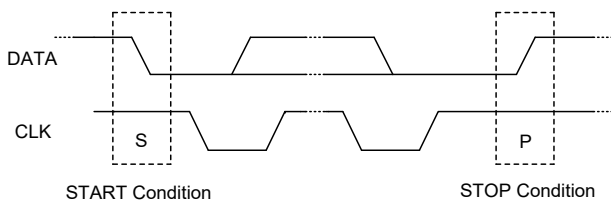
Figure 14. START and STOP Conditions
