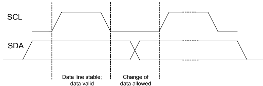
Figure 4. Bit Transfer
