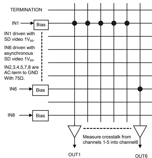
Figure 14. Test Configuration for Multi-Channel Crosstalk
