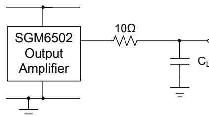
Figure 12. Driving Capacitive Loads
