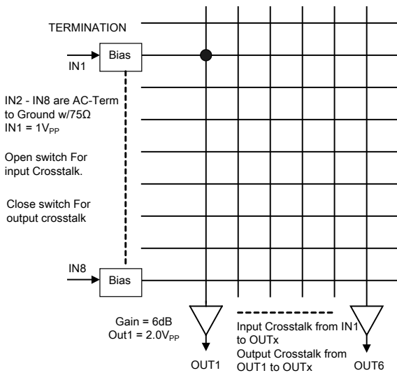
Figure 13. Test Configuration for Crosstalk
