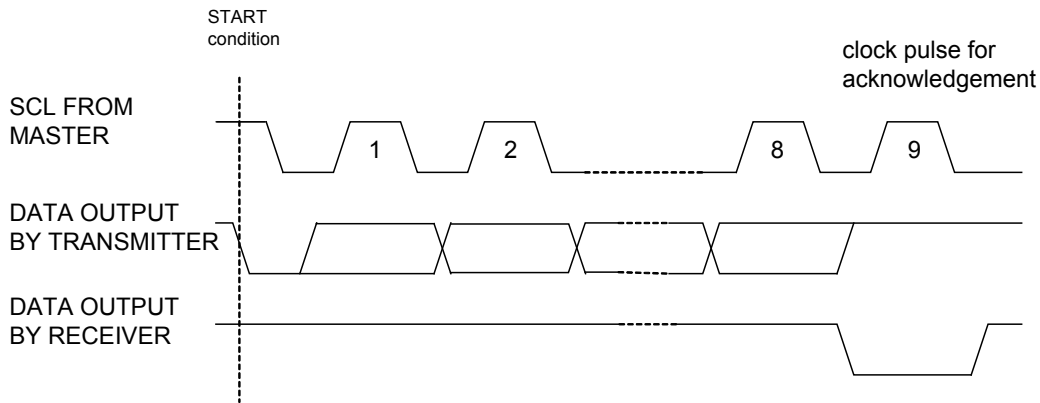
Figure 6. Acknowledgement on the I 2 C Bus
