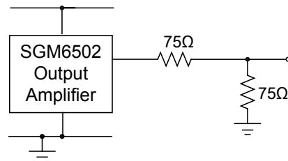
Figure 10. DC-Coupled Load Connection
