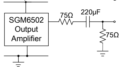
Figure 11. AC-Coupled Load Connection
