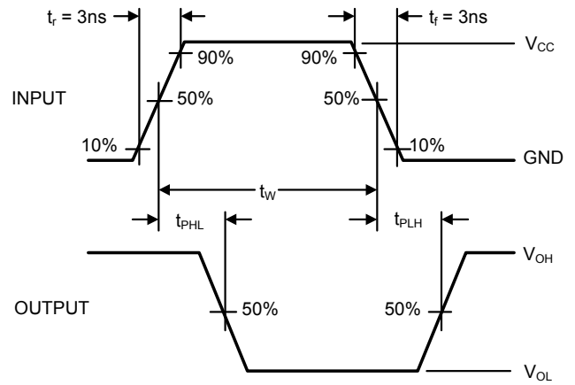
Figure 2. AC Waveforms
