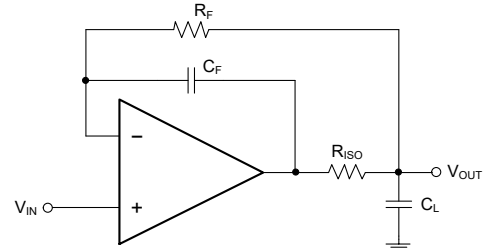
Figure 3. Circuit to Drive Heavy Capacitive Load
