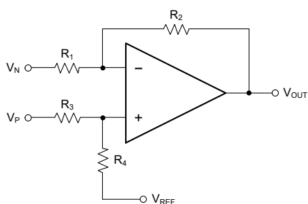
Figure 3. Difference Amplifier
