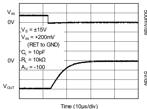
Negative Overload Recovery Time
