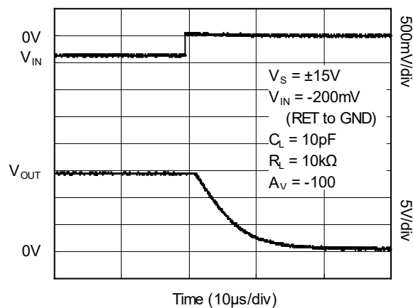
Positive Overload Recovery Time
