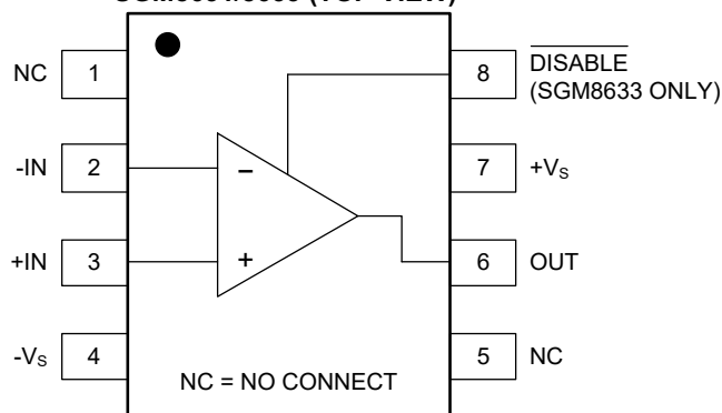
SGM8631/8633 (TOP VIEW)
