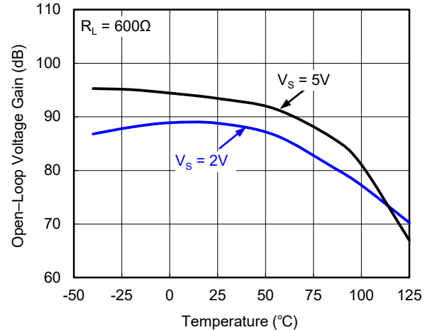
Open-Loop Voltage Gain vs. Temperature
