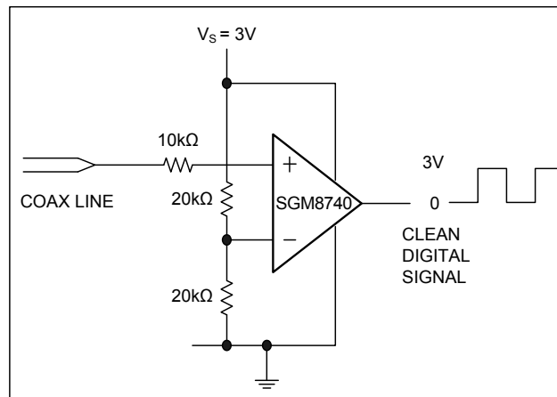
Figure 4. Line Receiver Application
