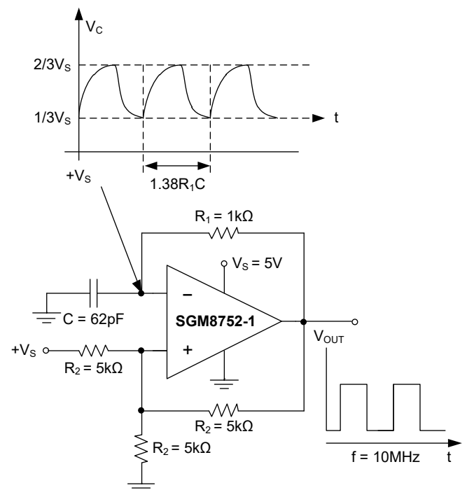
Figure 5. Relaxation Oscillator
