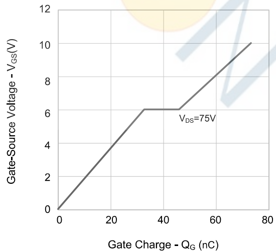
Figure 6. Gate Charge
