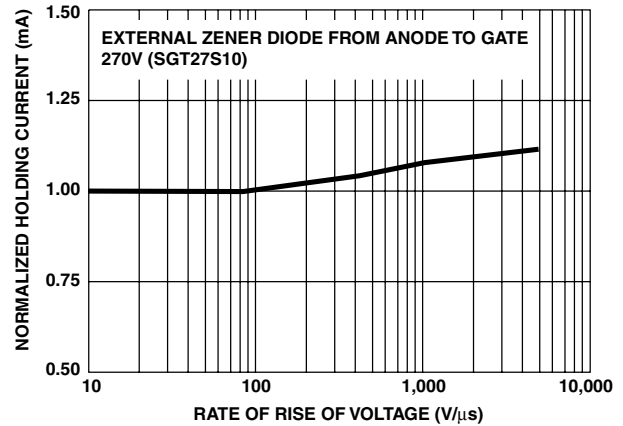
FIGURE 4. NORMALIZED V_{BO} vs dv/dt
