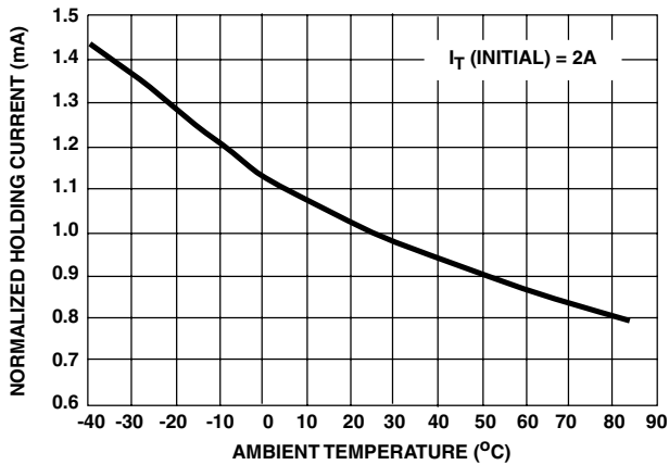
FIGURE 3. NORMALIZED HOLDING CURRENT vs TEMPERATURE
