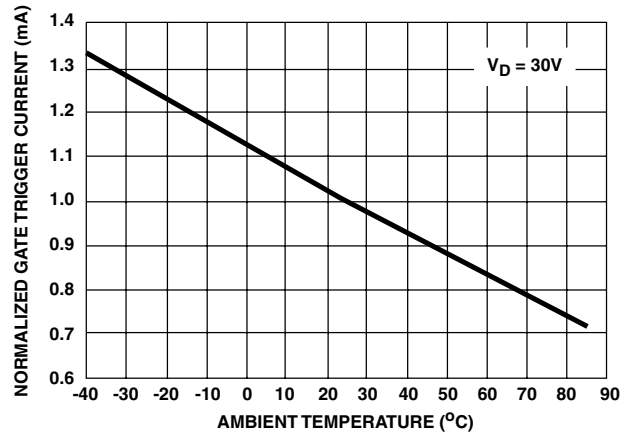
FIGURE 2. NORMALIZED GATE-TRIGGER CURRENT vs TEMPERATURE
