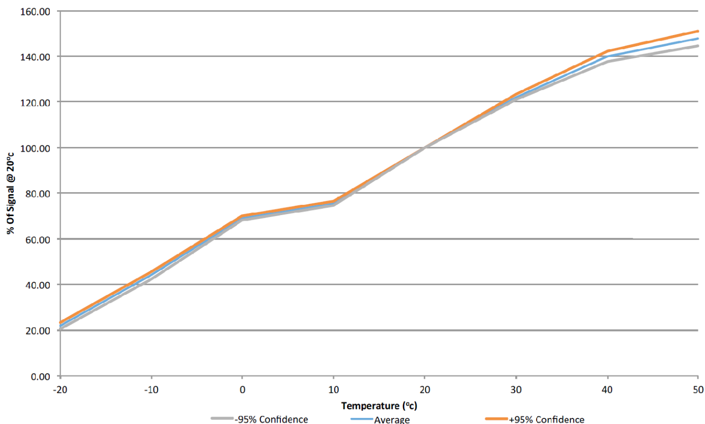
Output Temp Coefficient data
