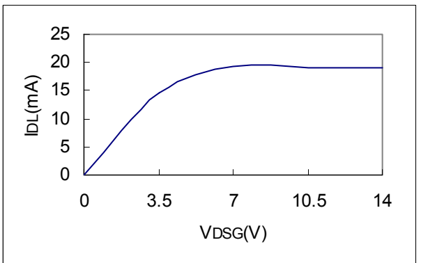
I_{DL} VS V_{D SG}
