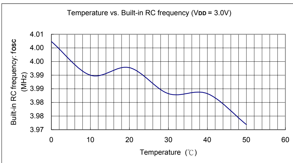
Temperature vs. Built-in RC fosc ( V_{DD} = 3.0V )
