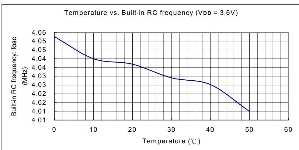
Temperature vs. Built-in RC fosc ( V_{DD} = 3.6V )
