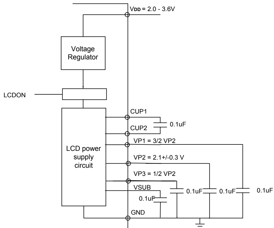
Figure 7. LCD Power Circuit Diagram
