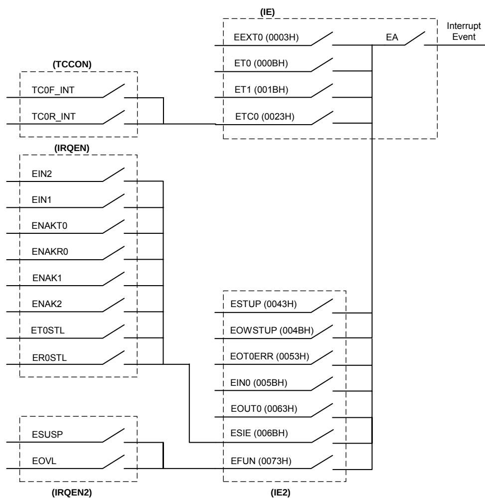
Figure 7-1. Interrupt Structure
