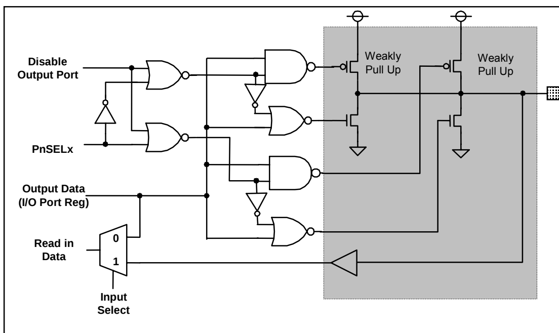
Figure 6-2. PORT Configuration-2
