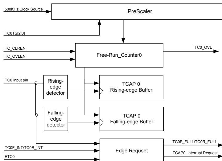
Figure 9-1. Function Block Diagram of Time Capture Function TCAP0
