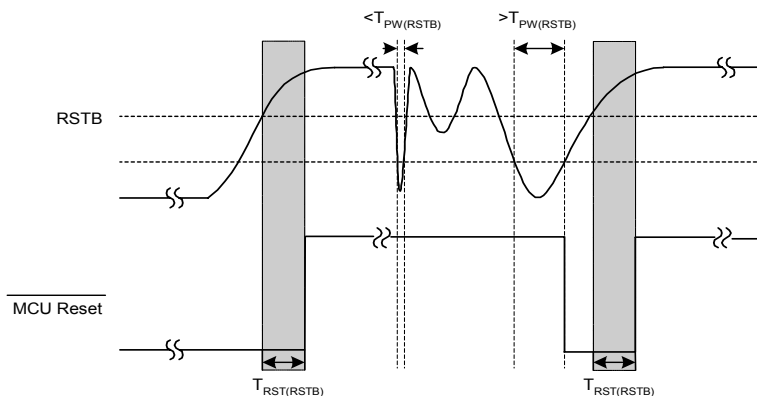
Figure 5-5. External Reset
