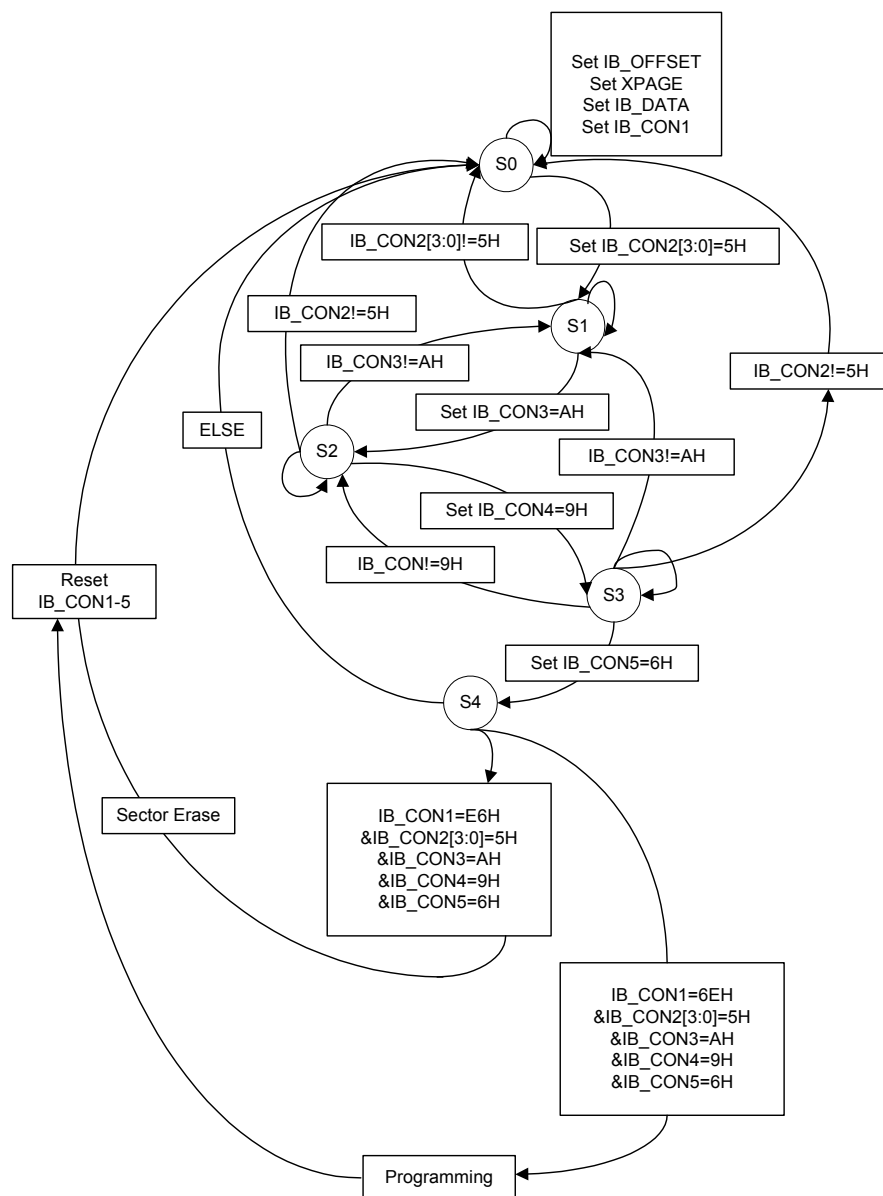
Figure 11-2. flash control flow
