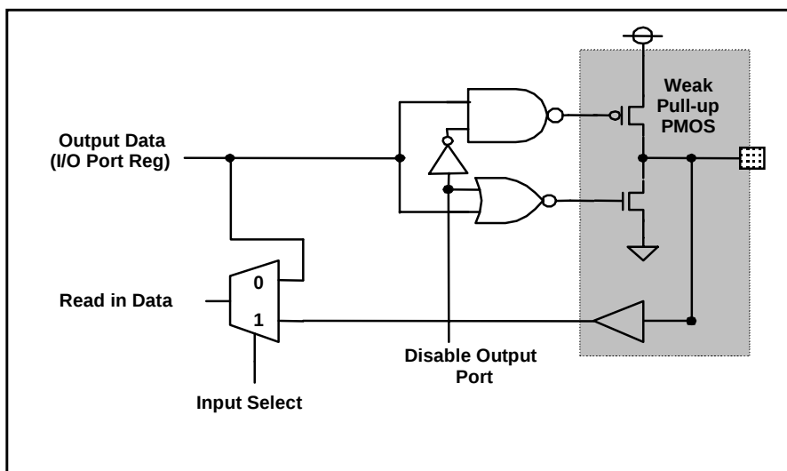
Figure 6-1. PORT Configuration-1
