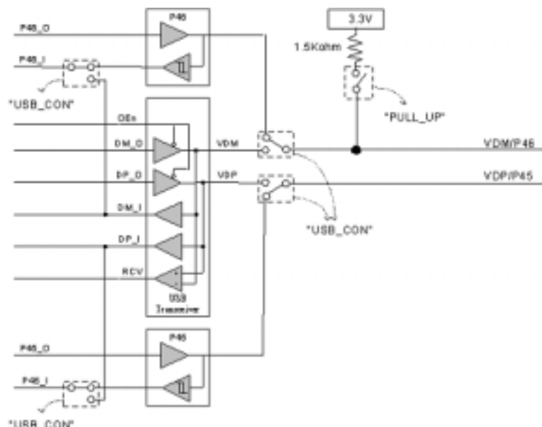
Figure 6-3. USB Configuration
