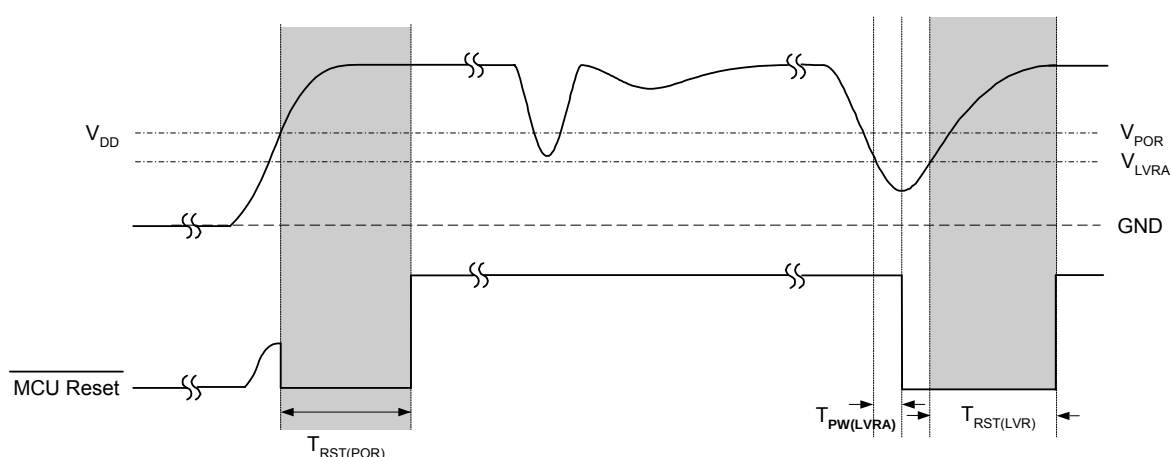
Figure 5-1. Power-on Reset and LVRA
