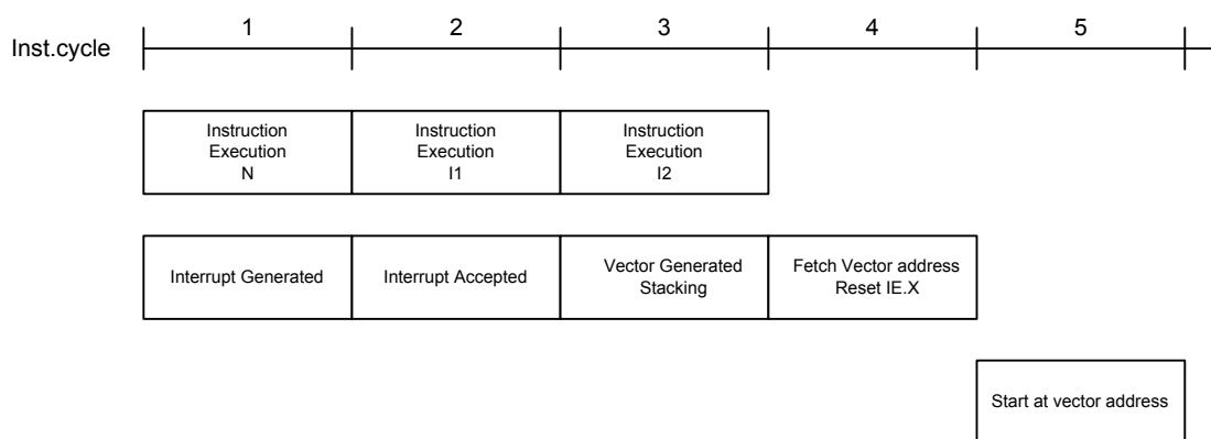
Figure 5. Interrupt Servicing Sequence Diagram
