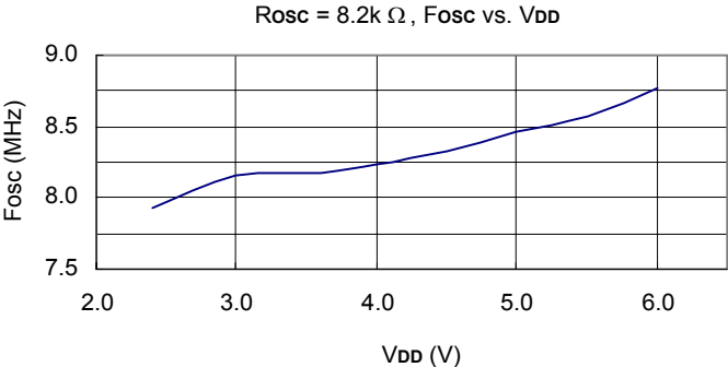
(c) Typical Internal RC oscillator Frequency stability vs. Operating Voltage: (for reference only)
