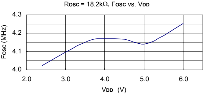
(b) Typical External RC oscillator Frequency vs. Operating Voltage: (for reference only)
