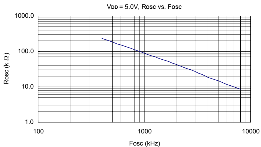
(a) Typical External RC oscillator Resistor vs. Frequency: (for reference only)
